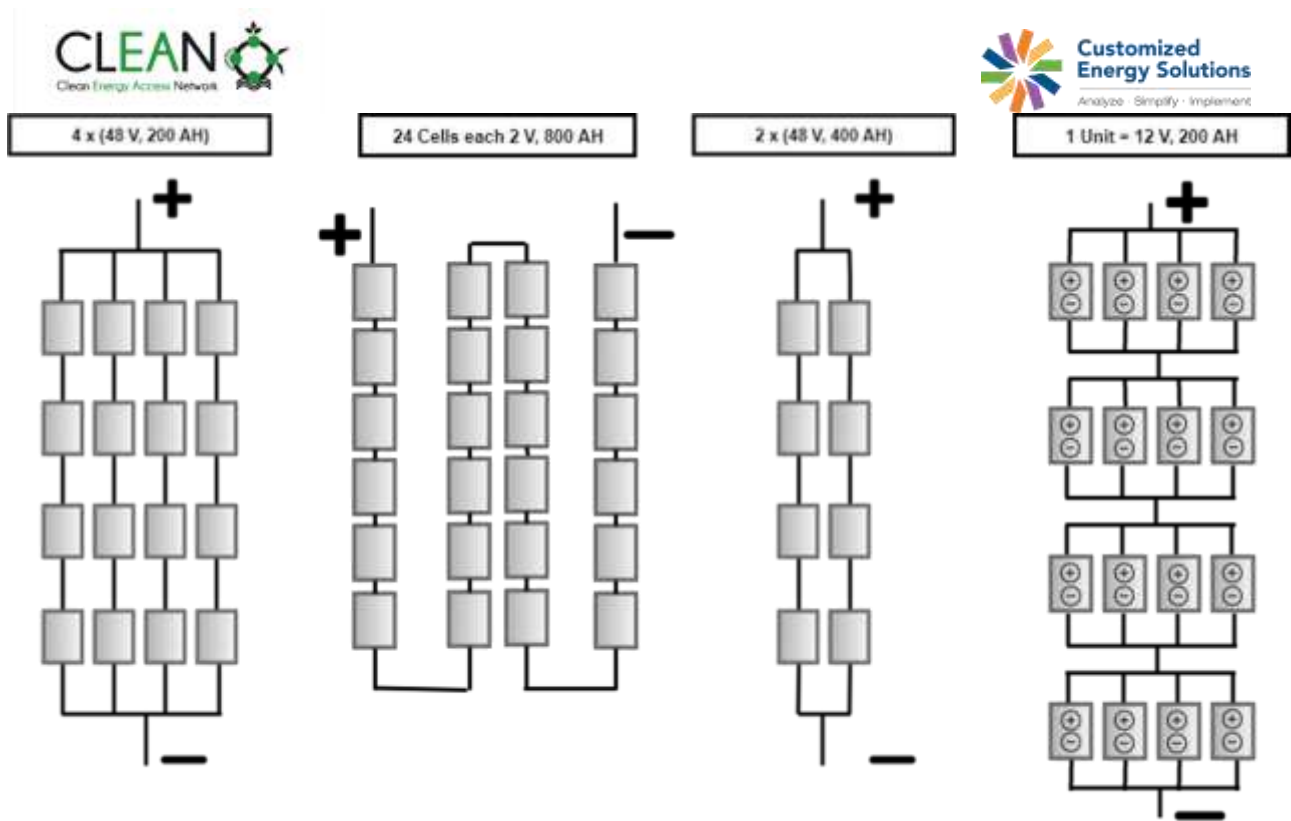
Figure 48 Parallel Connection of Lead Acid Cells & 12V batteries
