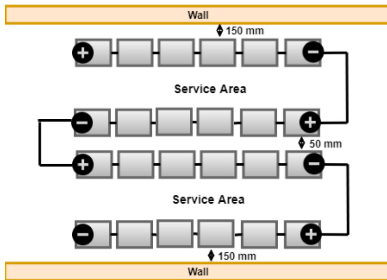
Figure 49 Layout of lead acid cells in a battery room (source: CES)
