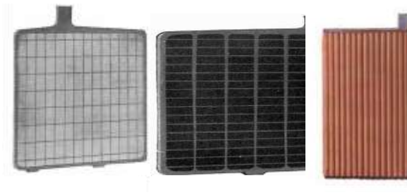
Figure 20 Construction of Flooded Lead Acid Batteries
