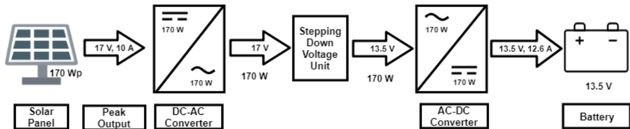
Figure 37 Block Diagram representing components of MPPT in a solar PV plant (source: CES)
