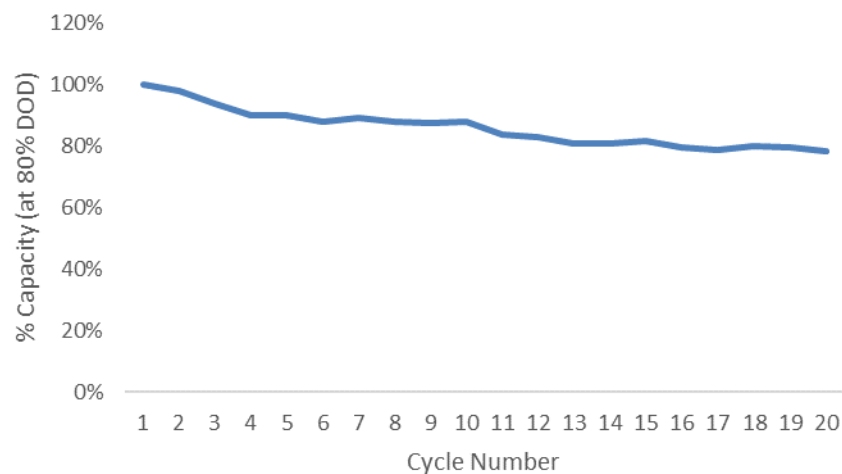
Figure 57 Ah Output in % of a flooded tubular battery at 80% DOD (source: CES)
